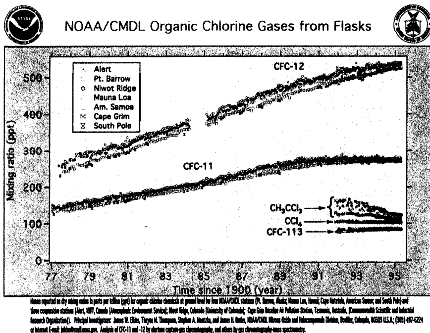
Figure (24) Measured Mixing Ratios in pptv, 1977–1995, for \text{CCl}_3\text{F} (CFC-11), \text{CCl}_2\text{F}_2 (CFC-12), \text{CCl}_2\text{FCClF}_2 (CFC-113), \text{CH}_2\text{CCl}_3 and \text{CCl}_4 .
