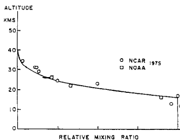
Figure (6) Mixing ratios for \text{CCl}_3\text{F} observed in 1975 by research groups from NCAR (o) [12] and NOAA ( \square ) [11] normalized to tropospheric value as 1.0. The solid line is the calculated value with diffusion coefficient C in Figure 3 [4].
